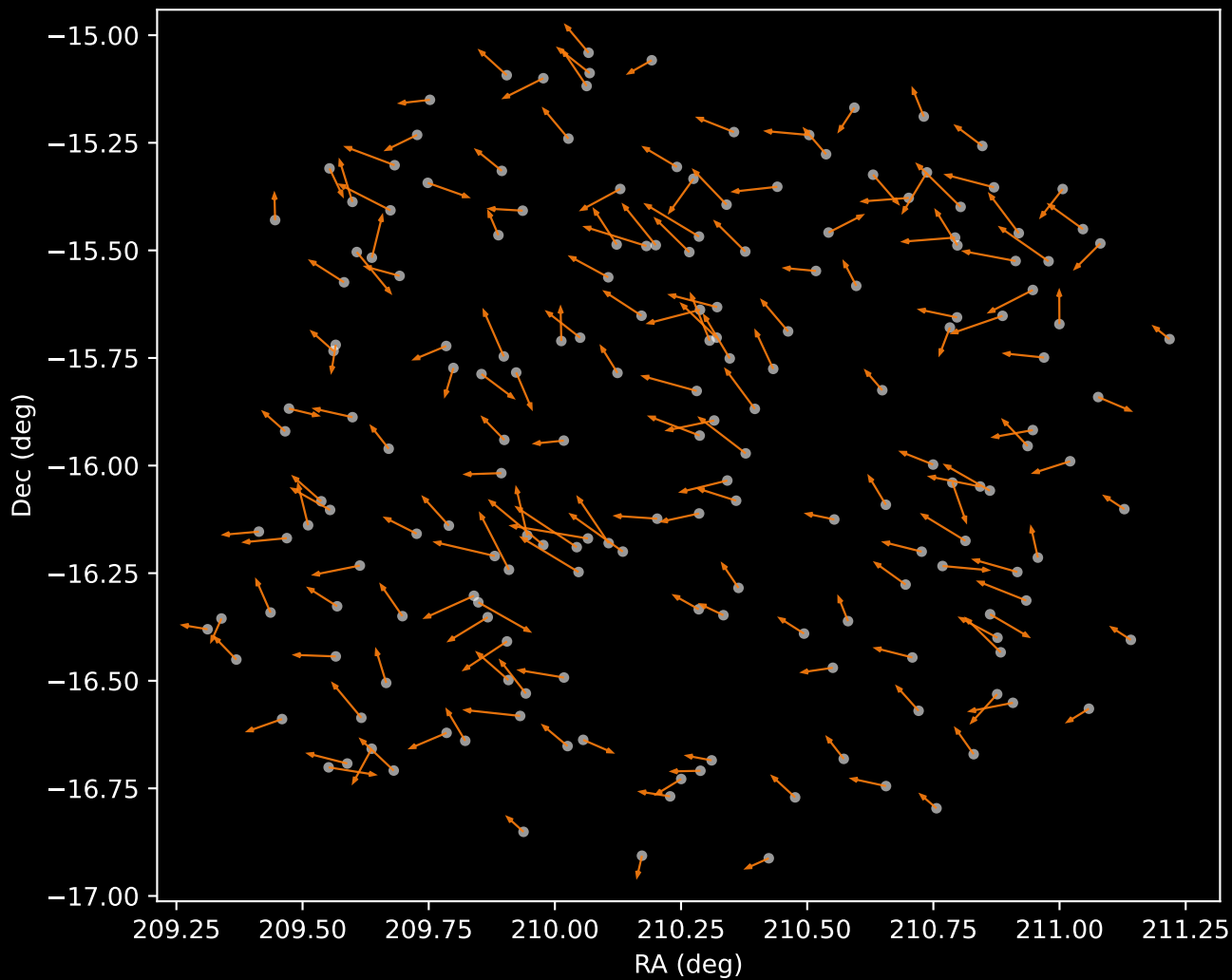
GALAH DR4 Cluster 2 Proper Motion Vectors (n=186)
