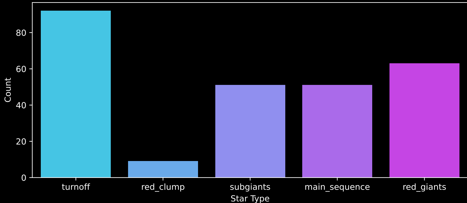
GALAH DR4 Field: [8686] Count plot of Star Type
