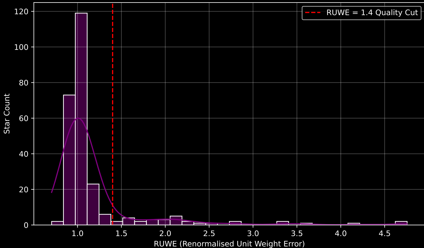
GALAH DR4 Field [8686] RUWE Distribution (n= 254)
